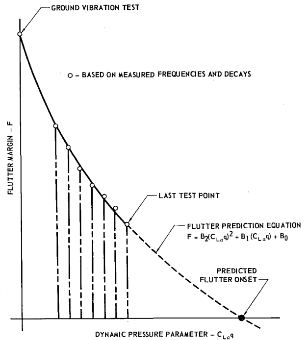
Fig. 5 Application of flutter margin technique.
