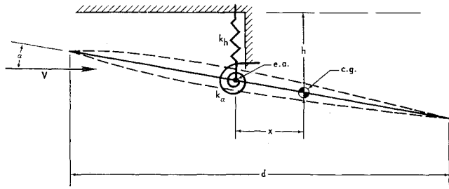
Fig. 3 Schematic of simple bending/torsion idealization.
