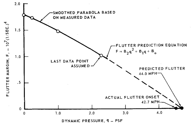
Fig. 12 Flutter model wing: prediction of flutter onset from measured data at subcritical speeds.
